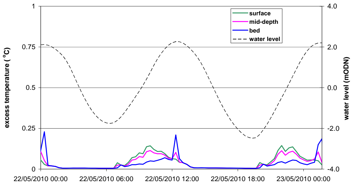
Figure 3.14 Predicted excess temperature variation at the Centrica intake, developed layout, neap tide, constant wind
