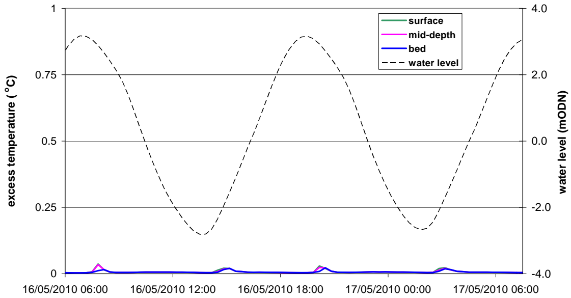
Figure 3.9 Predicted excess temperature variation at the Centrica intake, existing layout, spring tide, constant wind
