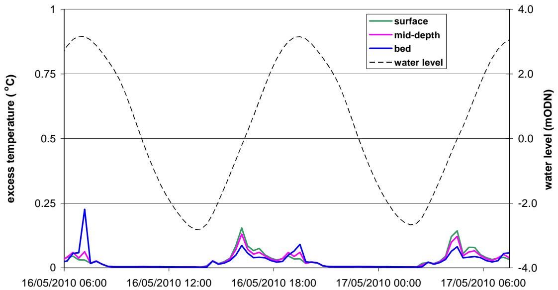
Figure 3.12 Predicted excess temperature variation at the Centrica intake, developed layout, spring tide, constant wind
