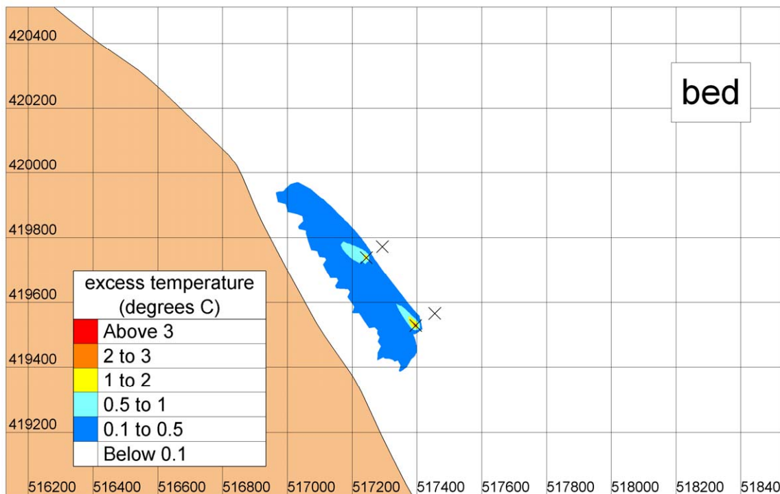
Figure 3.4 Predicted thermal dispersion patterns at Low Water, existing layout, spring tide, calm conditions
