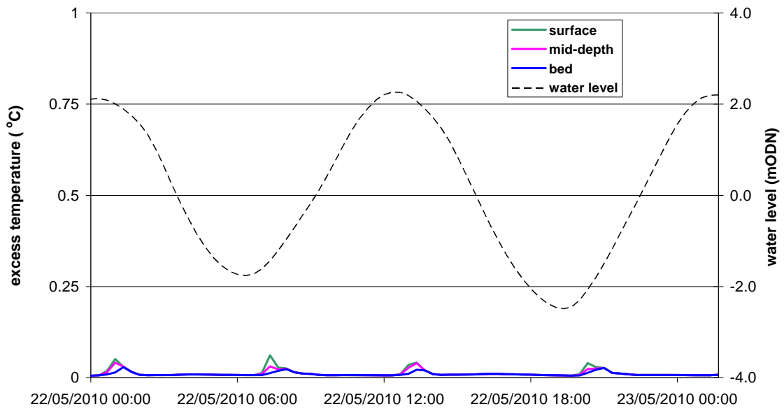
Figure 3.10 Predicted excess temperature variation at the Centrica intake, existing layout, neap tide, constant wind
