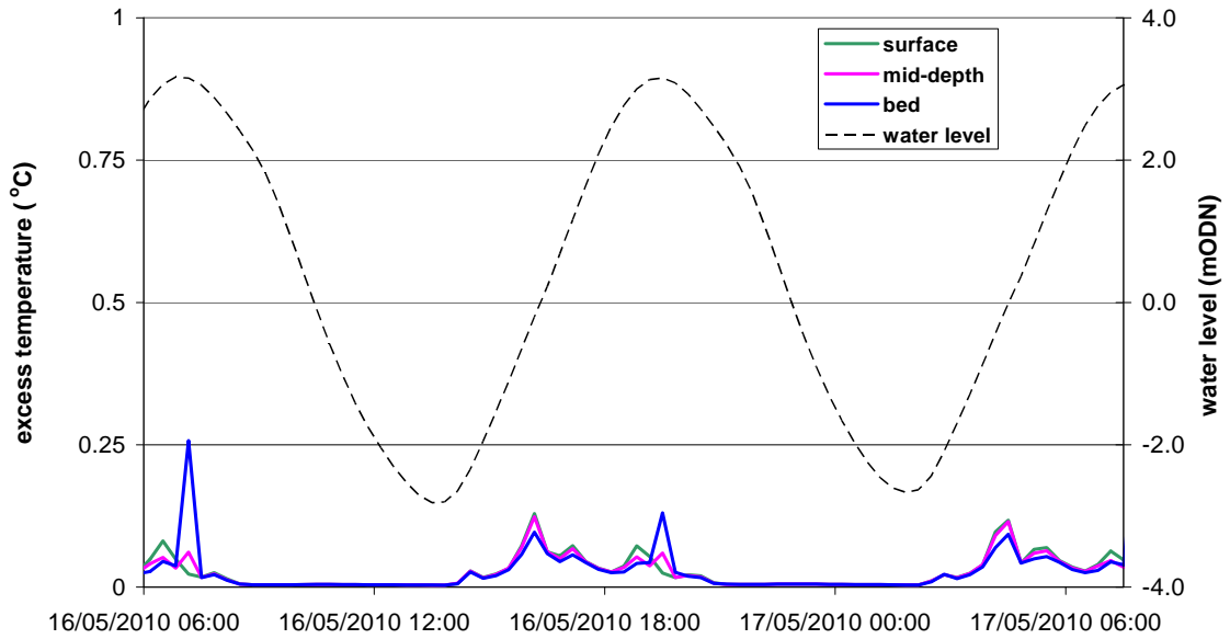
Figure 3.11 Predicted excess temperature variation at the Centrica intake, developed layout, spring tide, calm
