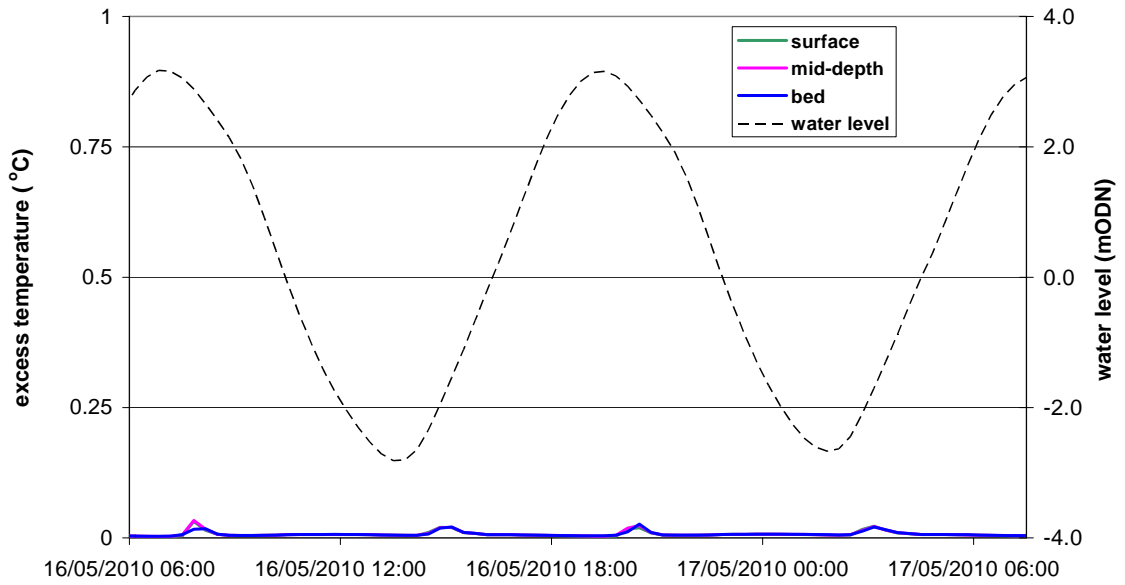
Figure 3.7 Predicted excess temperature variation at the Centrica intake, existing layout, spring tide, calm conditions
