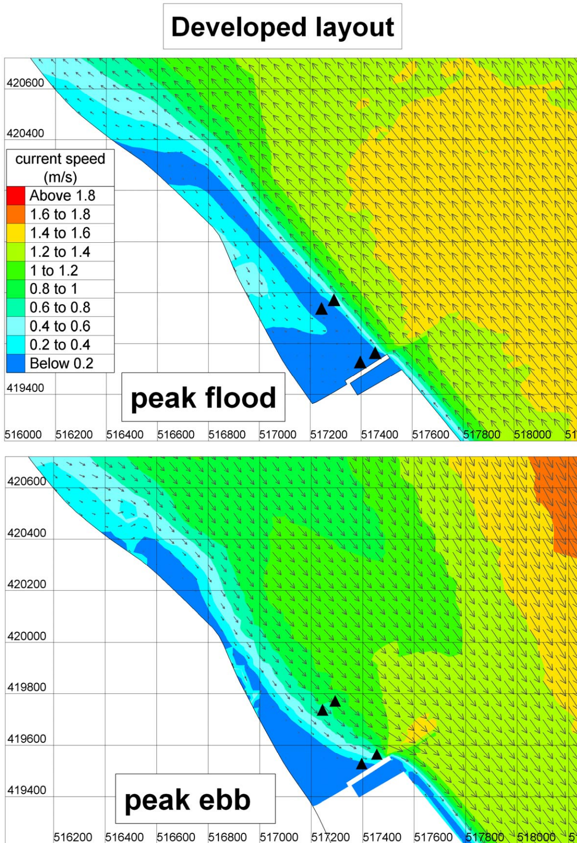
Figure 3.2b Predicted current patterns, spring tide, proposed developed condition
