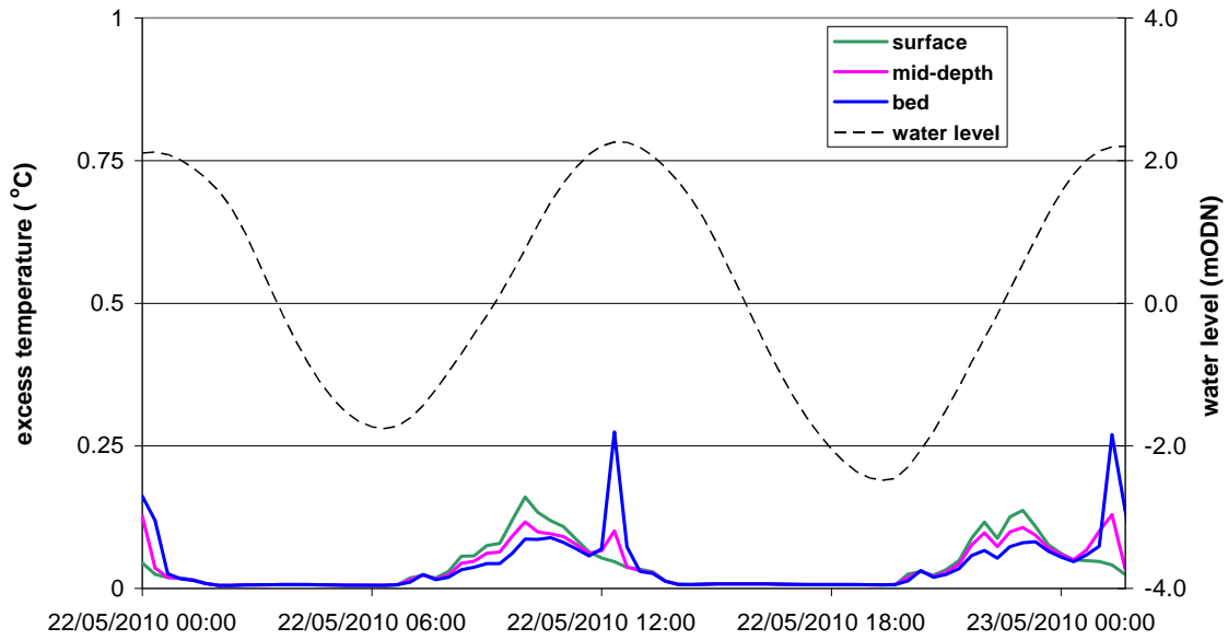
Figure 3.13 Predicted excess temperature variation at the Centrica intake, developed layout, neap tide, calm
