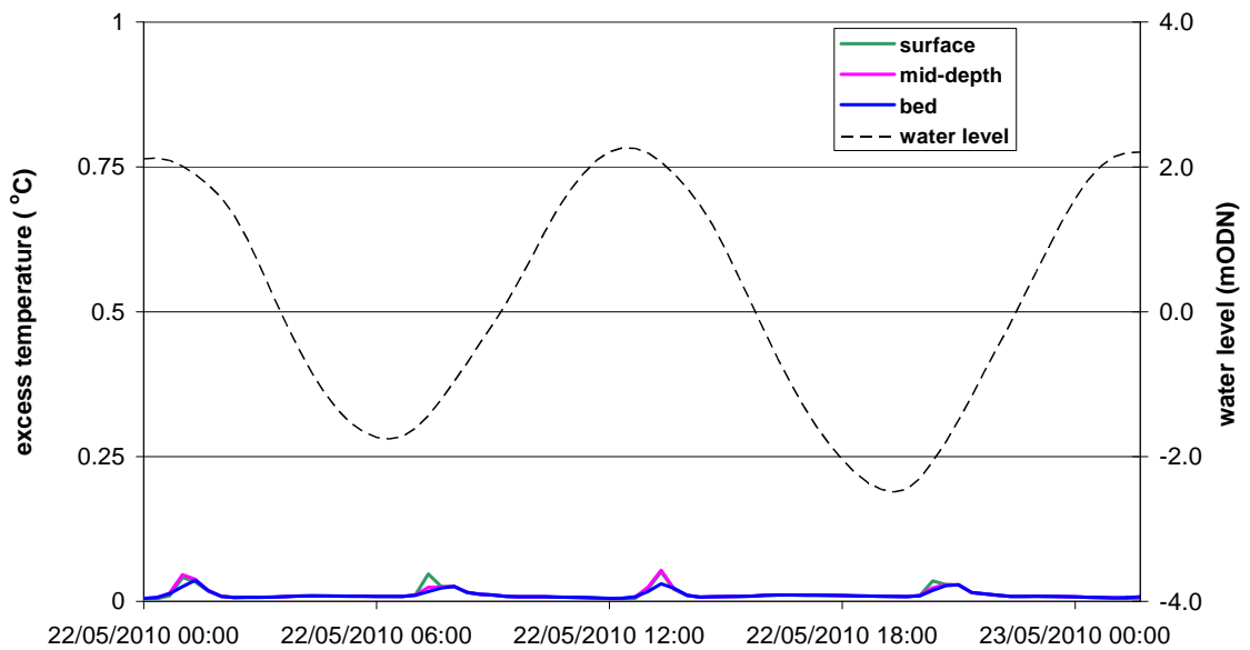
Figure 3.8 Predicted excess temperature variation at the E.ON intake, existing layout, neap tide, calm conditions
